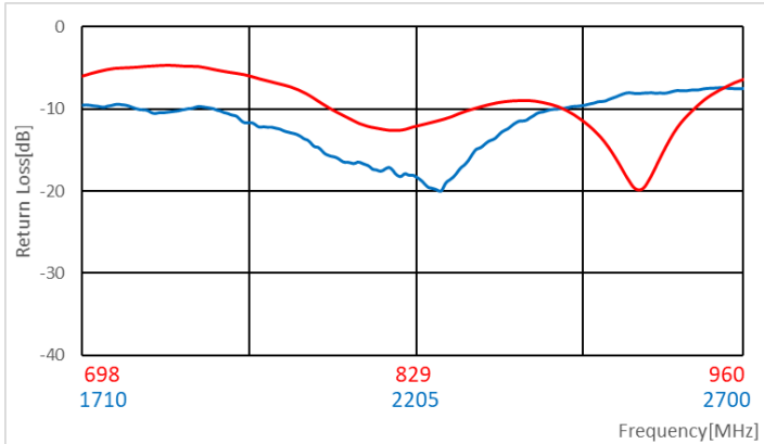
Return Loss
