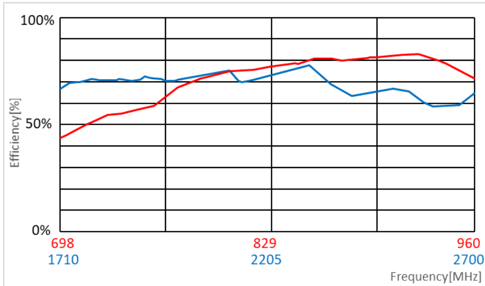
Efficiency
