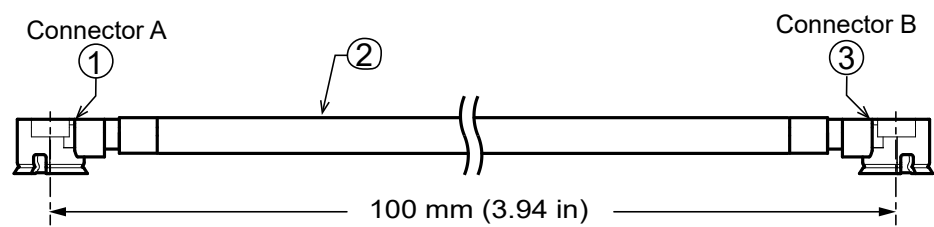
Figure 1. Product Dimensions for the CSG-UFFR-100-UFFR Cable Assembly
