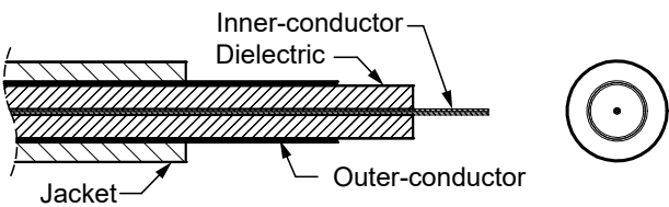
Figure 3. Coaxial Cable Cutaway Diagram
