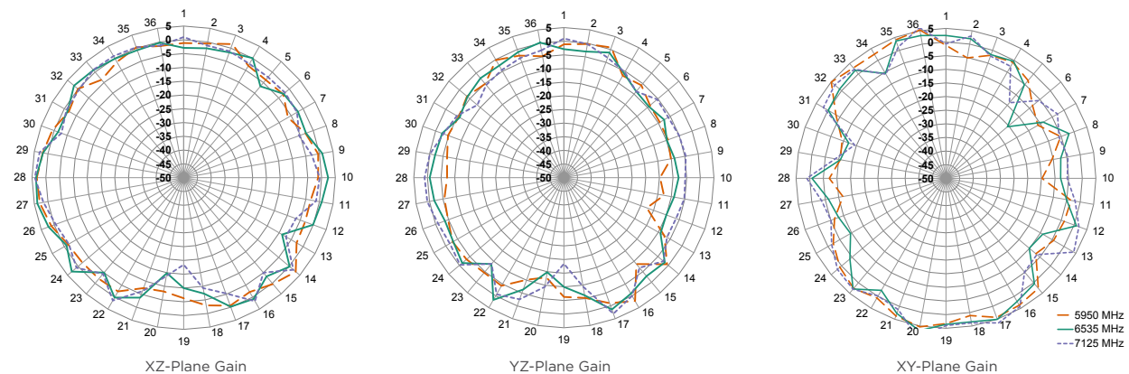
Figure 7. Radiation Patterns for ANT-W63-FPC-LH Series Antenna
