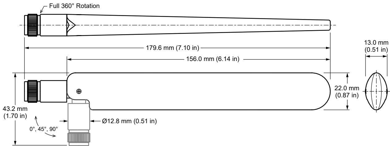
Figure 1: ANT-W63WS4-ccc Antenna Dimensions
