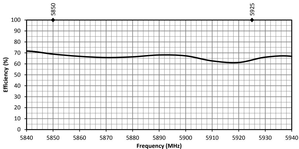
Figure 8. ANT-V2X-IPW1-NP Antenna Radiation Efficiency, Free Space
