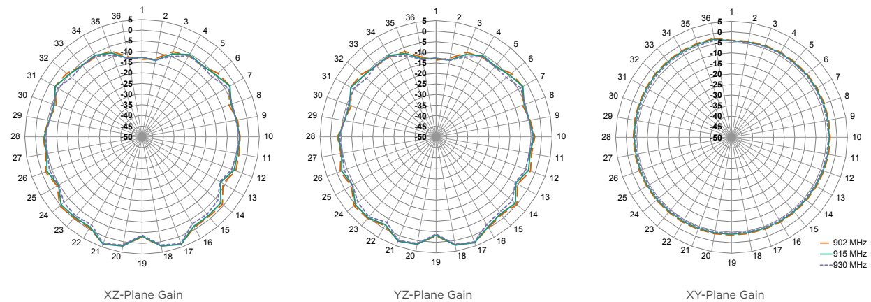
Figure 10. ANT-916-WRT Radiation Patterns, Free Space
