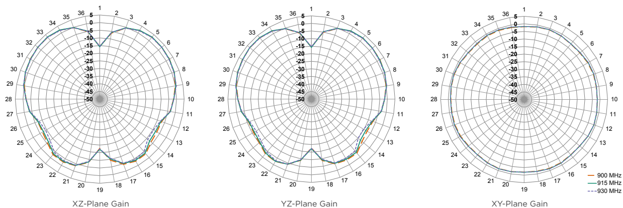
Figure 9. Radiation Patterns for ANT-8/9-MMG2-SMA Antenna
