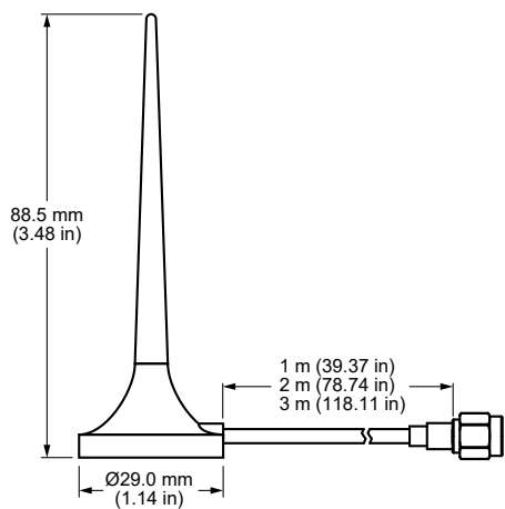
Figure 1. ANT-8/9-MMG2-SMA Series Antenna Dimensions
