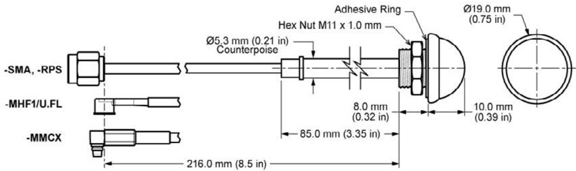
Figure 1. ANT-868-WRT Antenna Dimensions
