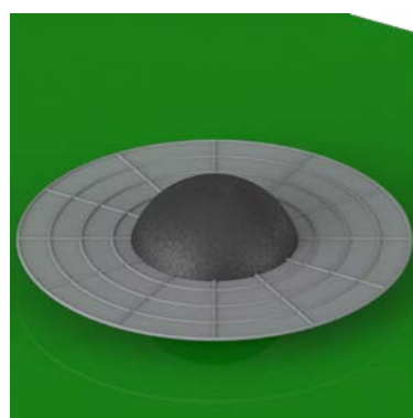
XY-Plane Gain
