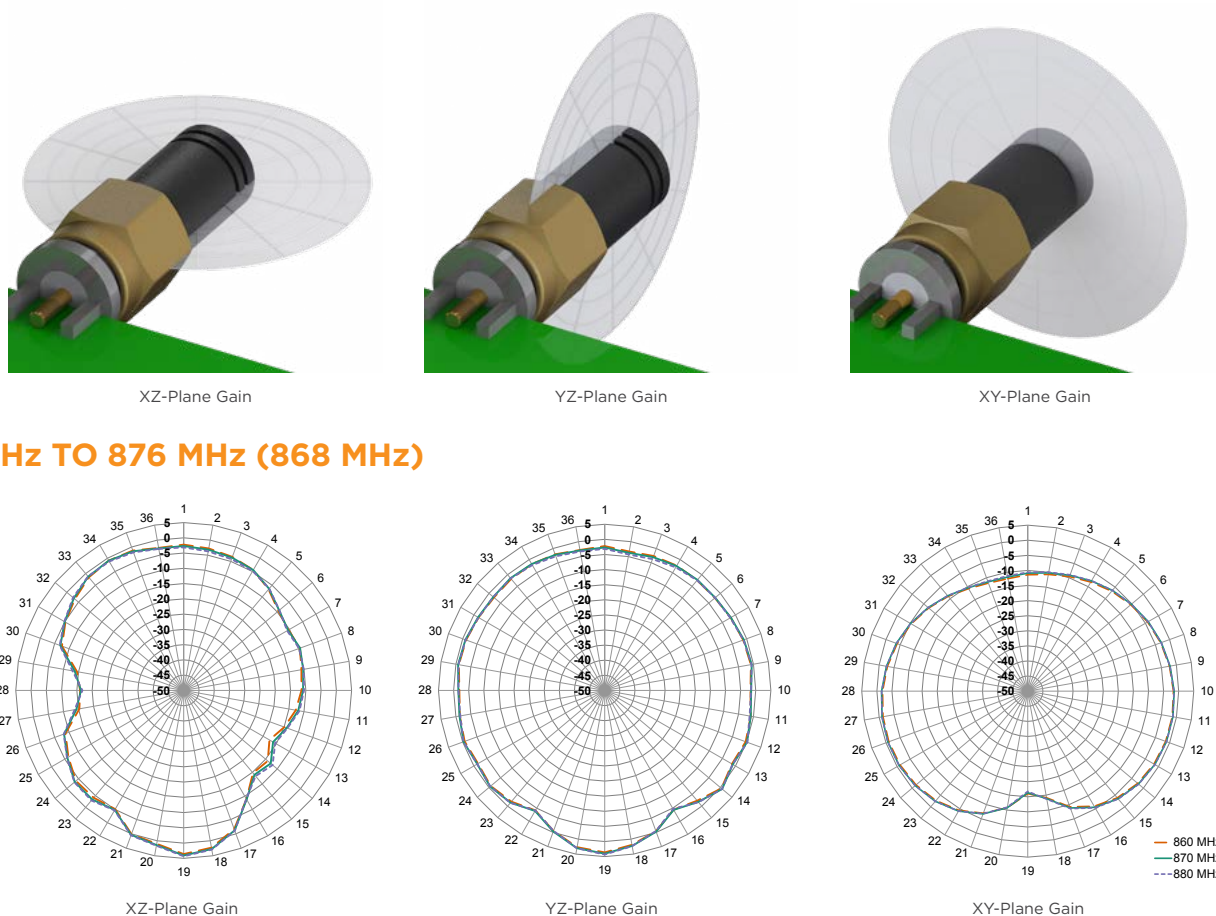
Figure 9. Radiation Patterns for ANT-868-NUB-ccc Antenna, Edge of ground Plane
