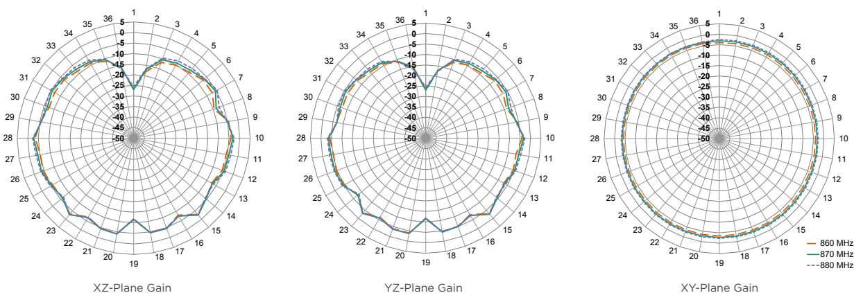
Figure 16. Radiation Patterns for ANT-868-NUB-ccc Antenna in Free Space
