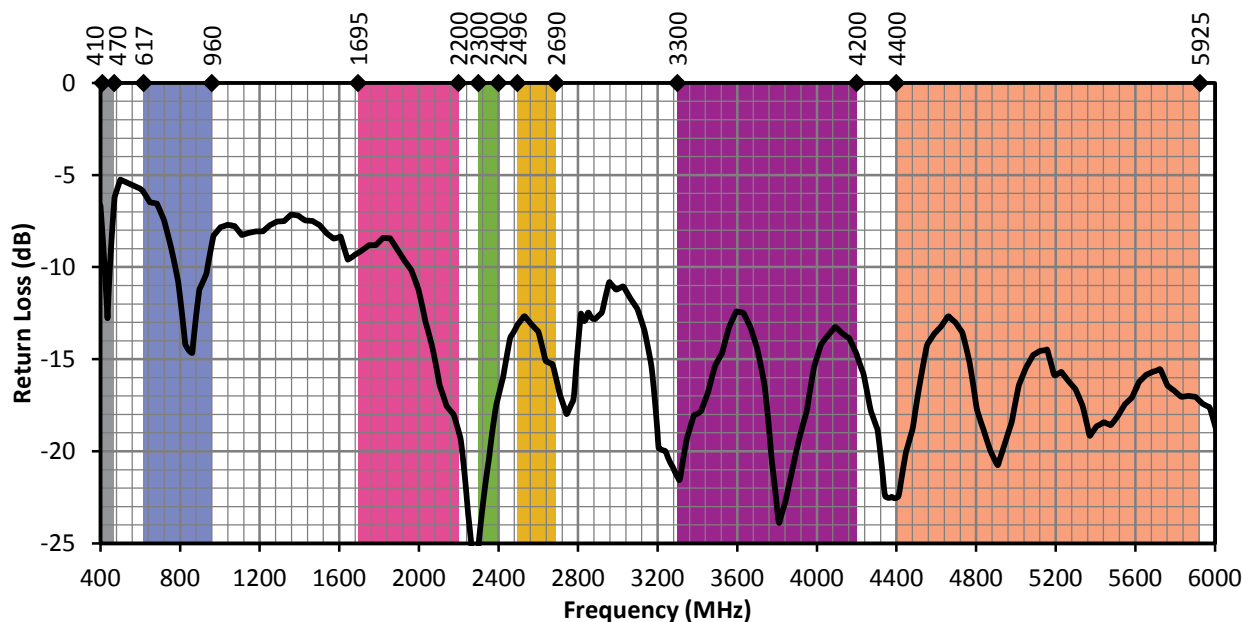
Figure 3. ANT-5GW-SPS1 Return Loss
