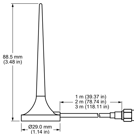
Figure 1. ANT-5GW-MMG2-SMA Series Antenna Dimensions
