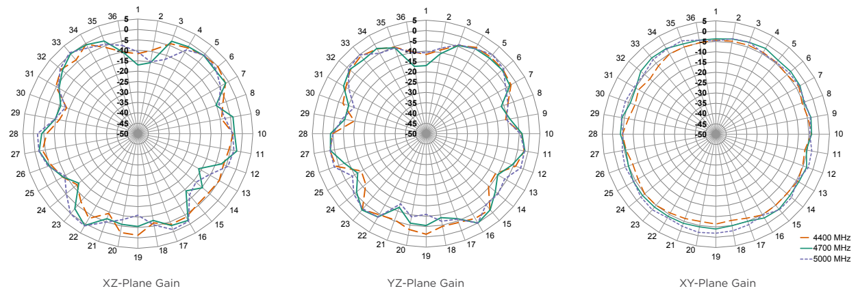
Figure 16 ANT-5GW-MMG2-SMA Radiation Patterns, Free Space Patterns
