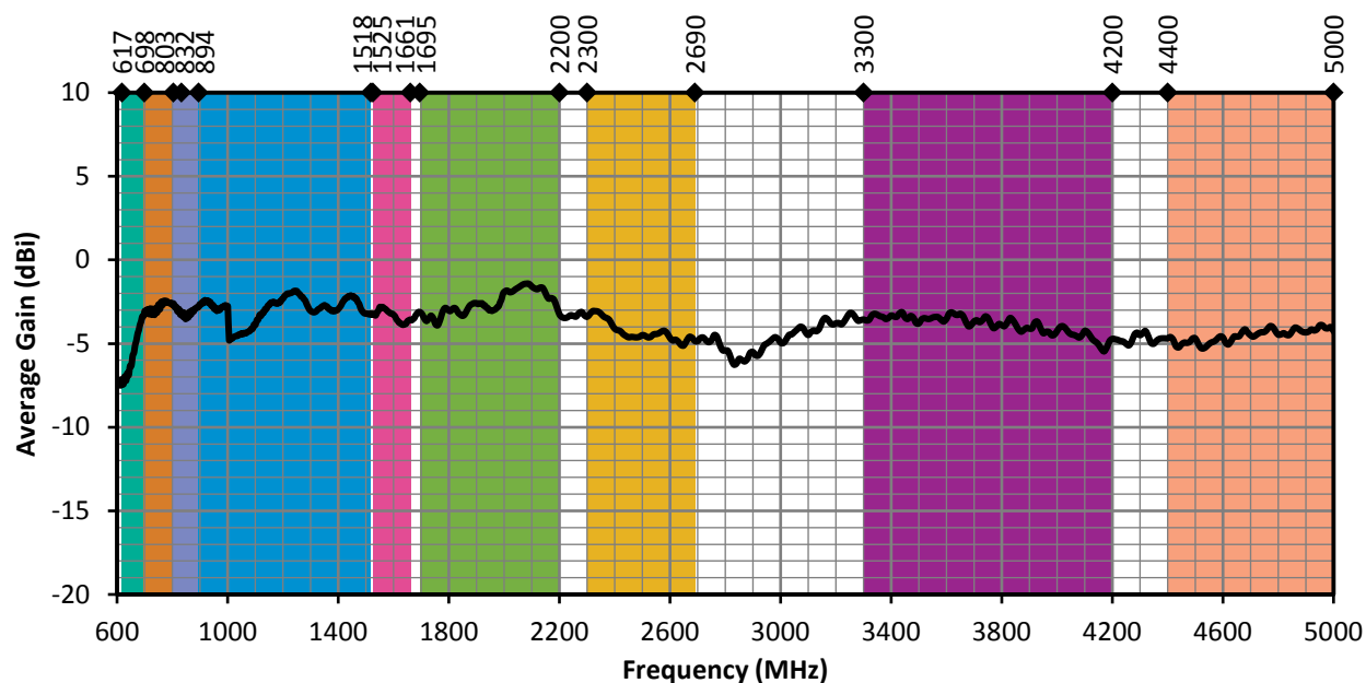
Figure 14. ANT-5GW-MMG2-SMA Antenna Average Gain, Free SpacePlane
