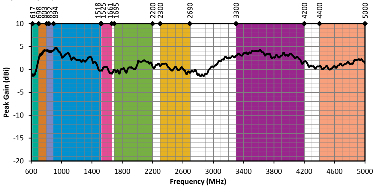
Figure 13. ANT-5GW-MMG2-SMA Peak Gain, Free SpacePlane
