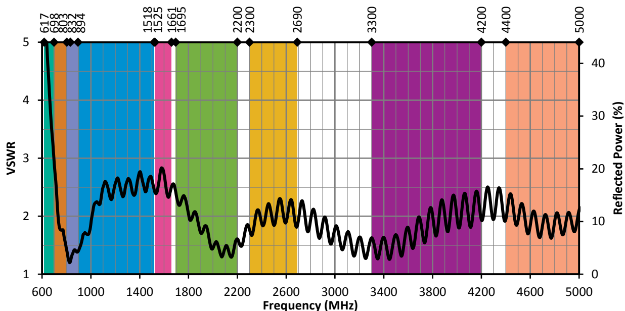
Figure 4. ANT-5GW-MMG2-SMA VSWR on Ground Plane
