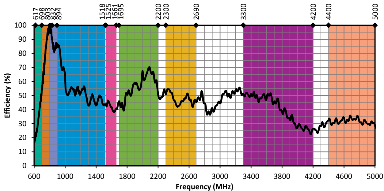
Figure 8. ANT-5GW-MMG2-SMA Antenna Efficiency on Ground Plane
