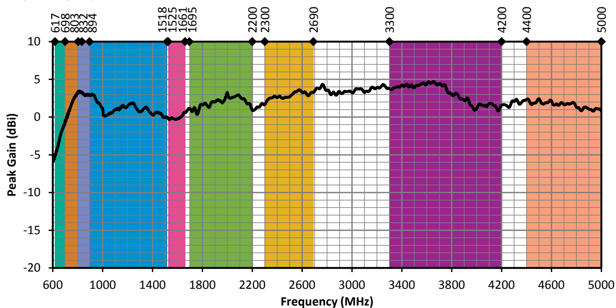
Figure 6. ANT-5GW-MMG2-SMA Peak Gain on Ground Plane
