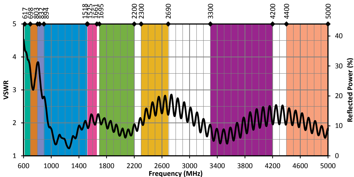
Figure 11. ANT-5GW-MMG2-SMA VSWR, Free Space
