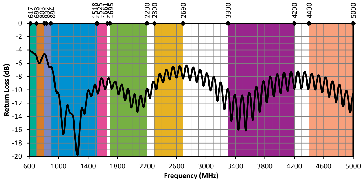
Figure 12. ANT-5GW-MMG2-SMA Return Loss, Free SpacePlane
