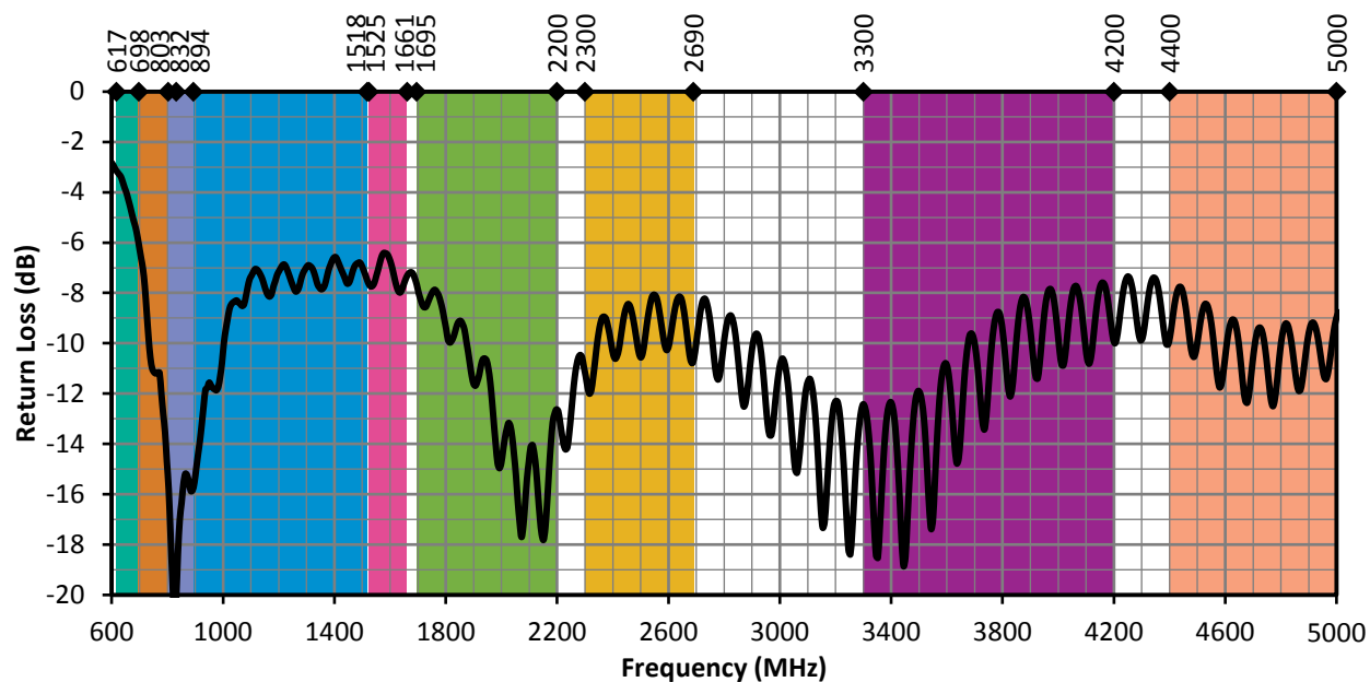
Figure 5. ANT-5GW-MMG2-SMA Return Loss on Ground Plane
