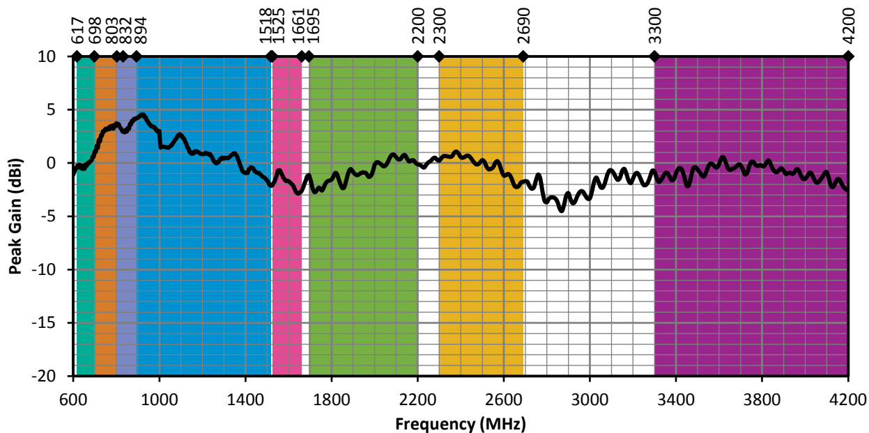
Figure 13. ANT-5GW-MMG1-SMA Peak Gain, Free Space
