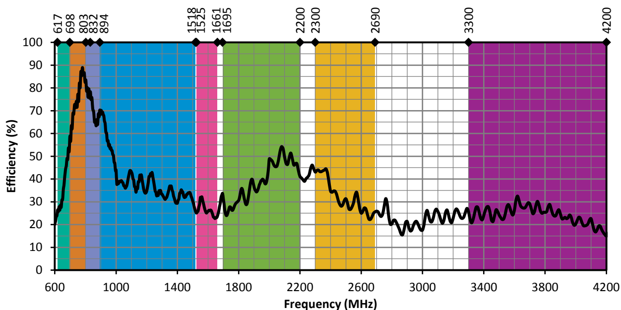
Figure 8. ANT-5GW-MMG1-SMA Antenna Efficiency on Ground Plane
