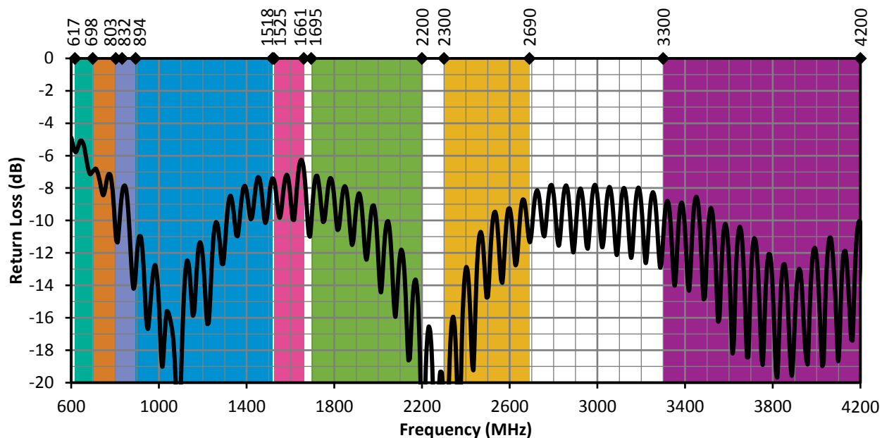
Figure 12. ANT-5GW-MMG1-SMA Return Loss, Free Space
