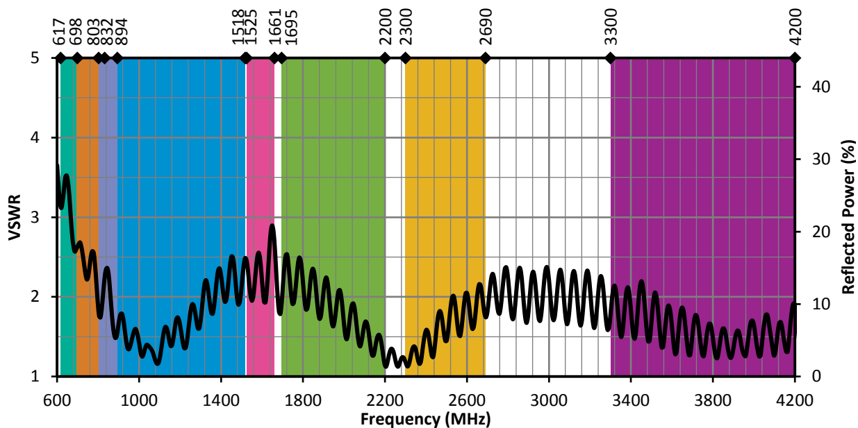
Figure 11. ANT-5GW-MMG1-SMA VSWR, Free Space
