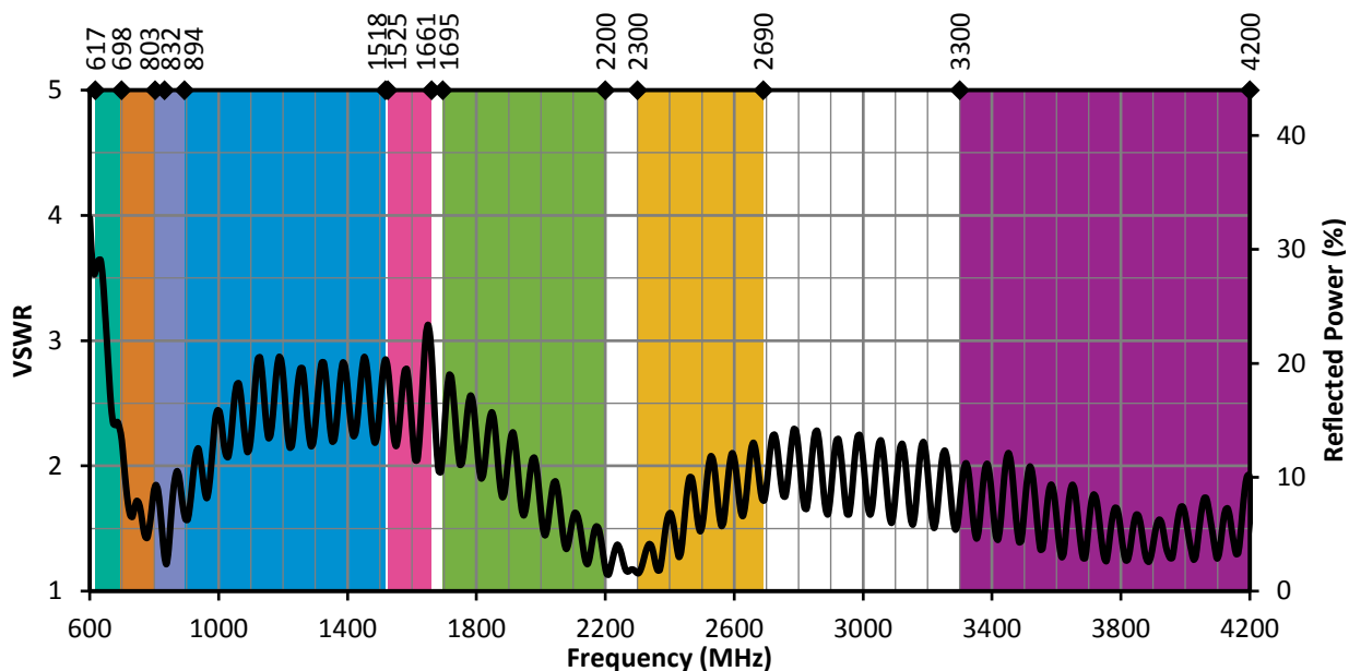
Figure 4. ANT-5GW-MMG1-SMA VSWR on Ground Plane
