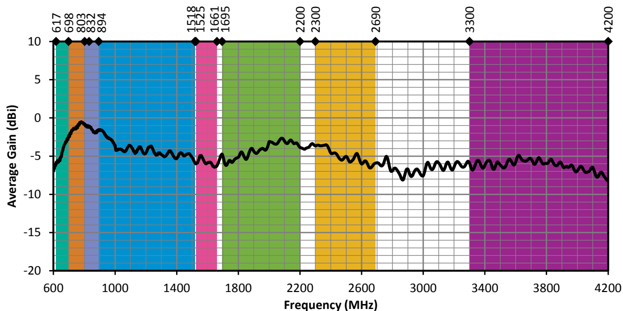
Figure 7. ANT-5GW-MMG1-SMA Antenna Average Gain on Ground Plane
