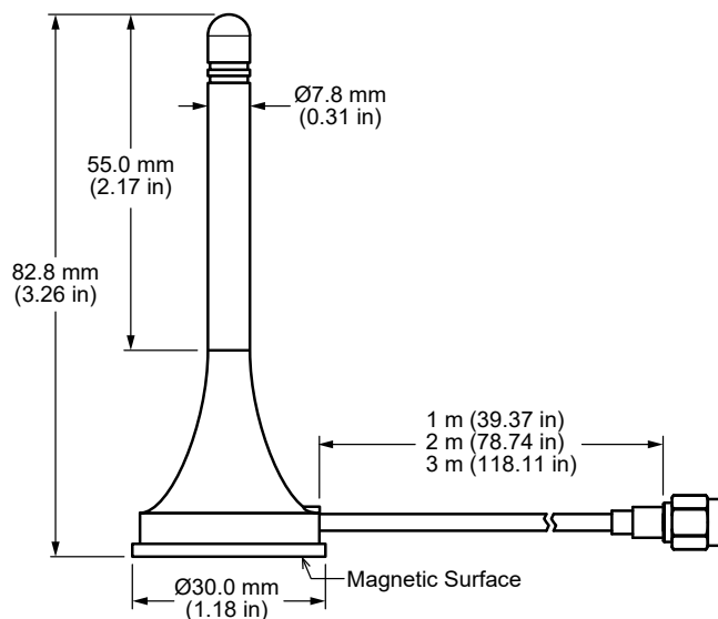
Figure 1. ANT-5GW-MMG1-SMA Series Antenna Dimensions
