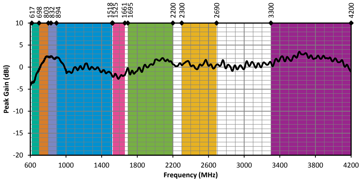
Figure 6. ANT-5GW-MMG1-SMA Peak Gain on Ground Plane
