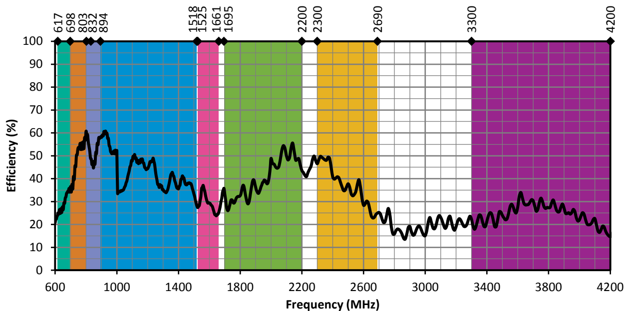
Figure 15. ANT-5GW-MMG2-SMA Antenna Efficiency, Free Space
