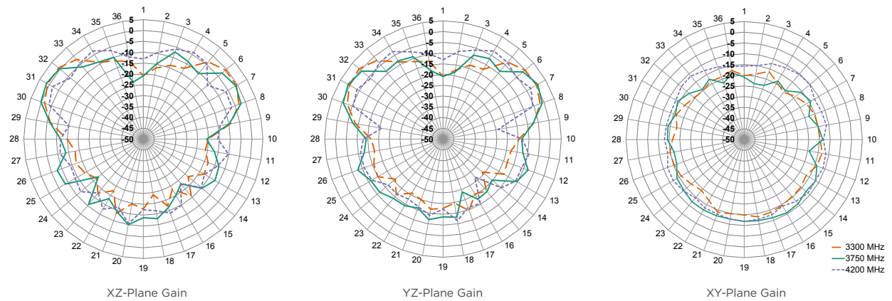
Figure 9. ANT-5GW-MMG1-SMA Radiation Patterns, on Ground Plane
