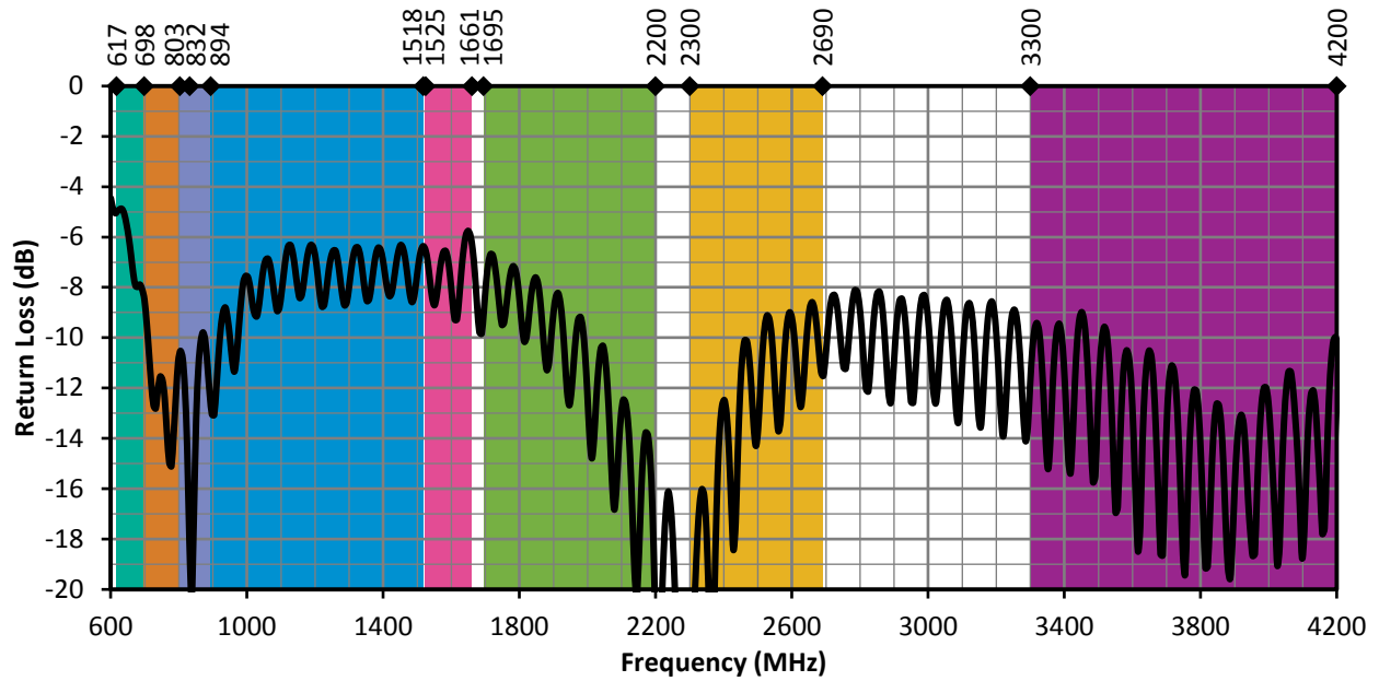
Figure 5. ANT-5GW-MMG1-SMA Return Loss on Ground Plane
