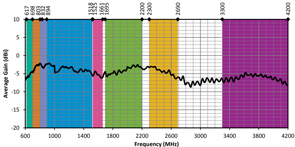
Figure 14. ANT-5GW-MMG1-SMA Antenna Average Gain, Free Space
