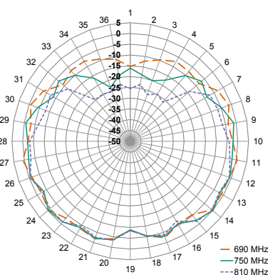
XY-Plane Gain
