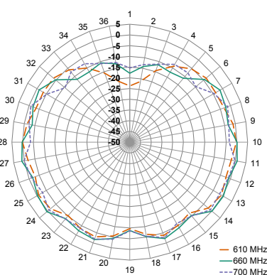
XY-Plane Gain
