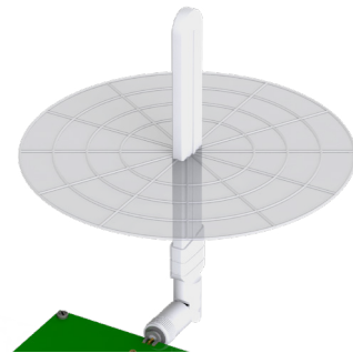
XY-Plane Gain
