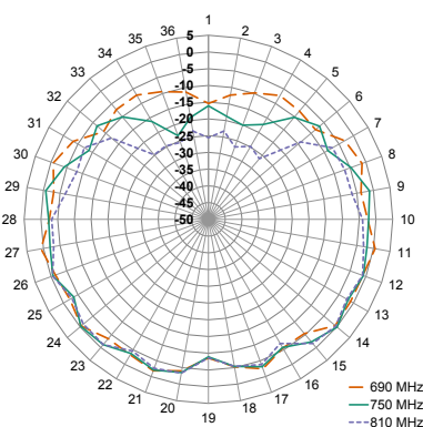
XY-Plane Gain
