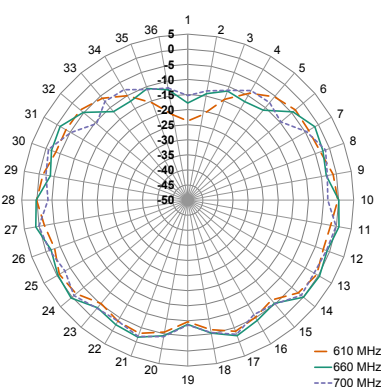
XY-Plane Gain
