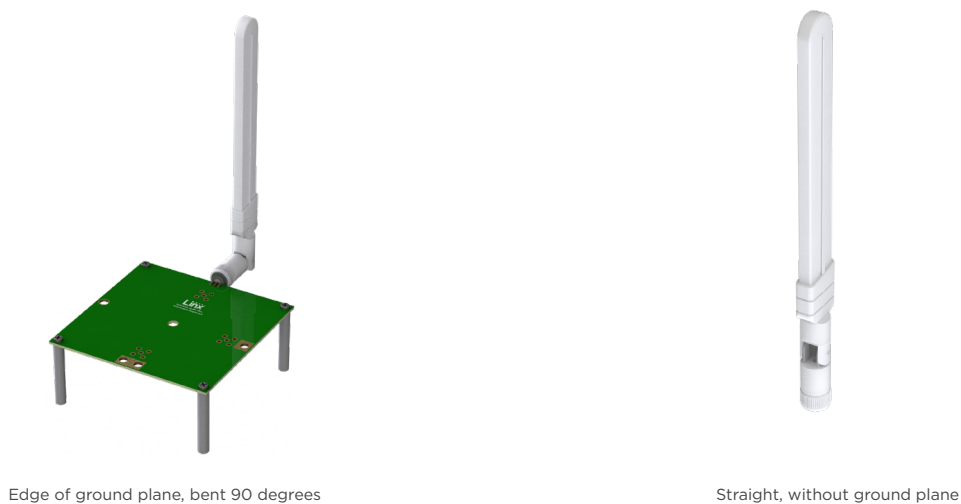
Figure 2. ANT-5GWWS4-ccc on evaluation PCB
