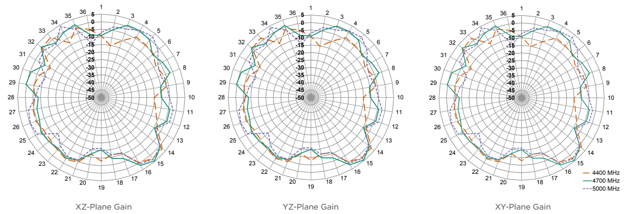
Figure 9. Radiation Patterns for ANT-5GWWS4-ccc, Edge-Bent
