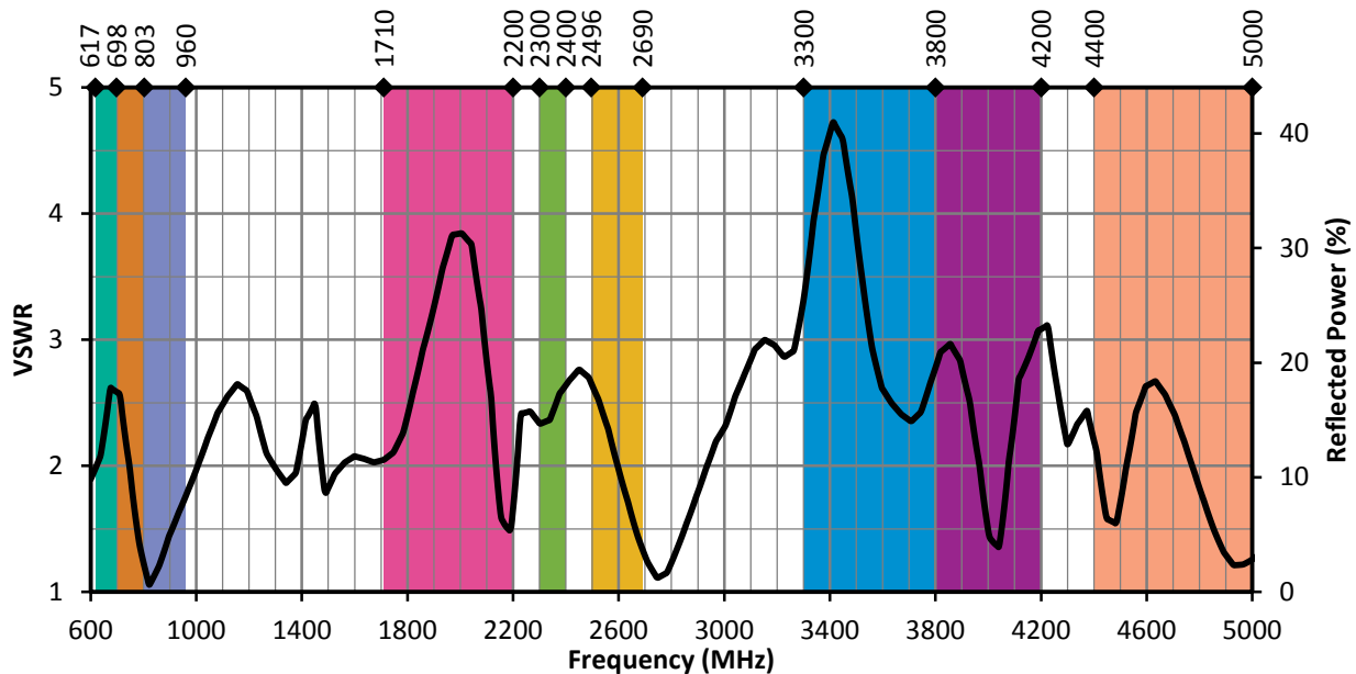
Figure 11. ANT-5GWWS4-ccc VSWR, Straight
