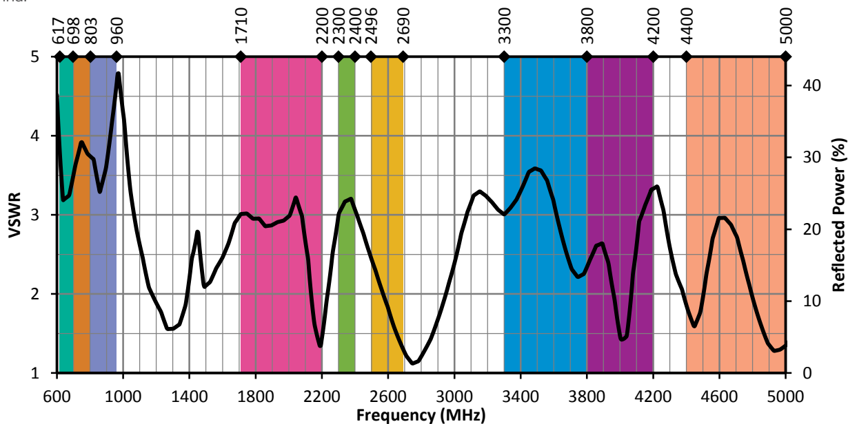
Figure 4. ANT-5GWWS4-ccc VSWR, Edge-Bent
