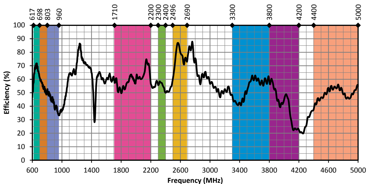
Figure 8. ANT-5GWWS4-ccc Antenna Efficiency, Edge-Bent
