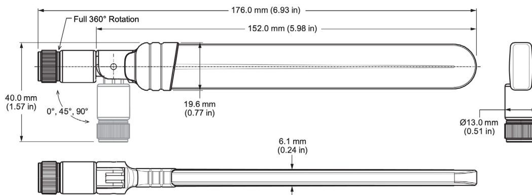
Figure 1. ANT-5GWWS4-ccc Antenna Dimensions
