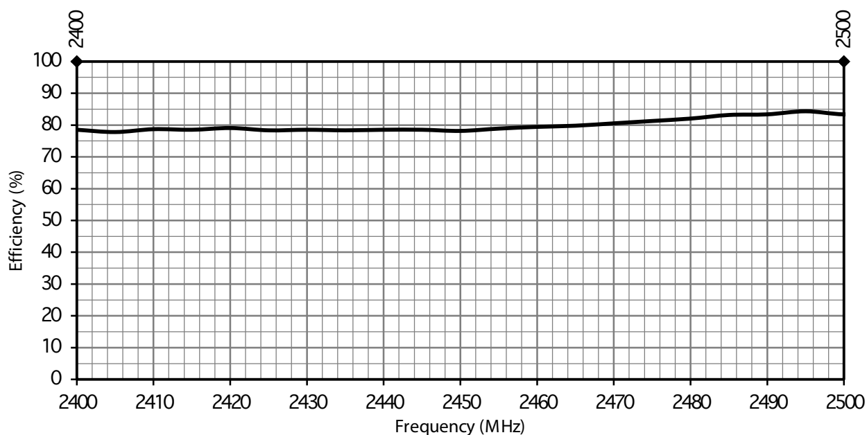
Figure 8. ANT-2.4-WRT-MON Antenna Radiation Efficiency
