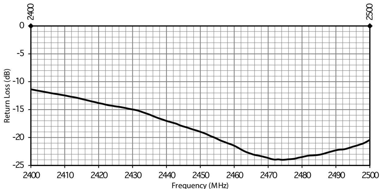
Figure 5. ANT-2.4-WRT-MON Return Loss
