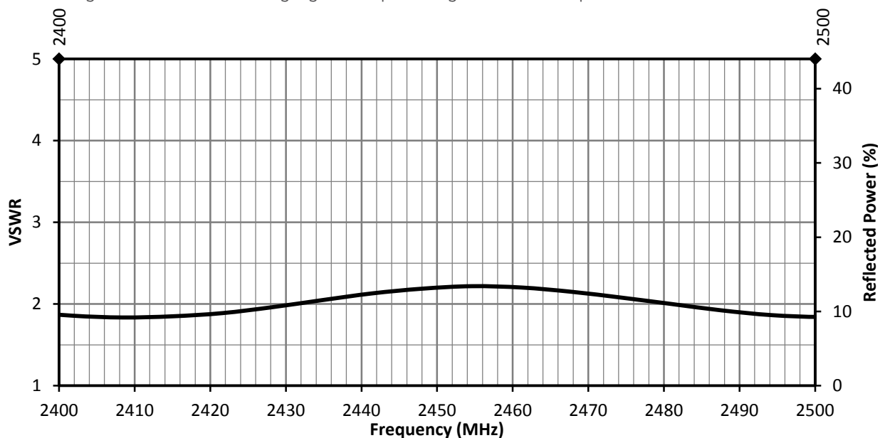
Figure 4. ANT-2.4-MMG2-SMA Antenna VSWR on Ground Plane
