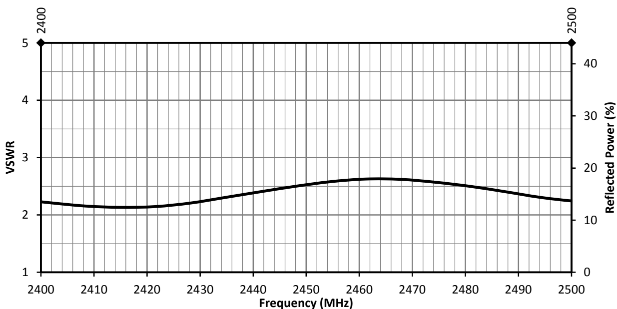
Figure 11. ANT-2.4-MMG2-SMA Antenna VSWR, Free Space
