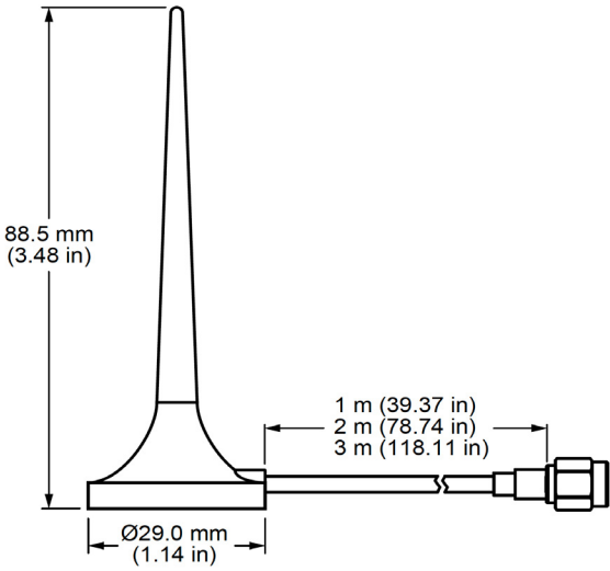
Figure 1. ANT-2.4-MMG2-SMA Series Antenna Dimensions
