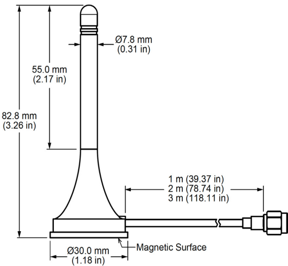
Figure 1. ANT-2.4-MMG1-SMA Series Antenna Dimensions
