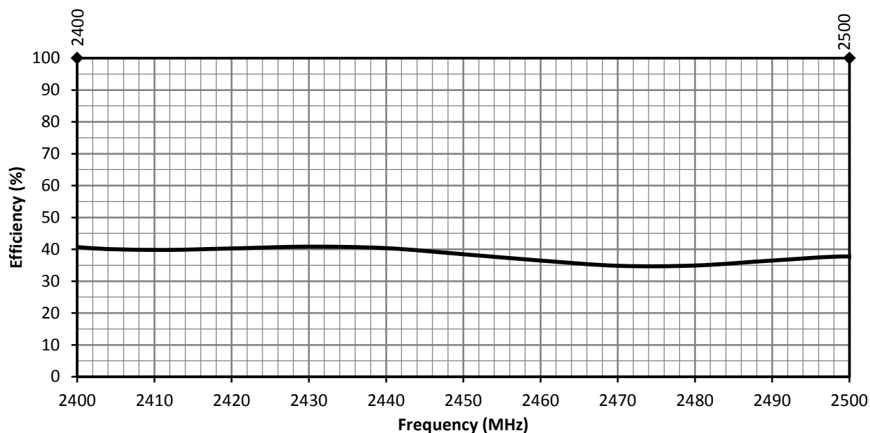
Figure 15. ANT-2.4-MMG1-SMA Antenna Radiation Efficiency, Free Space
