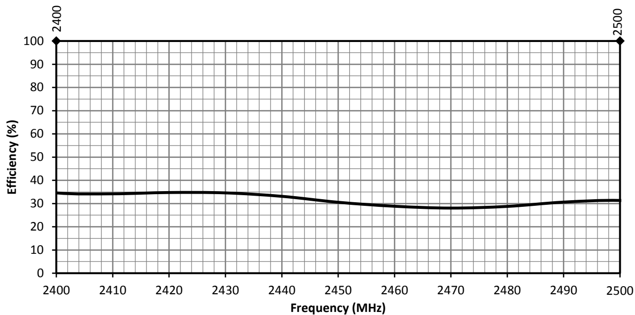
Figure 8. ANT-2.4-MMG1-SMA Antenna Radiation Efficiency on Ground Plane
