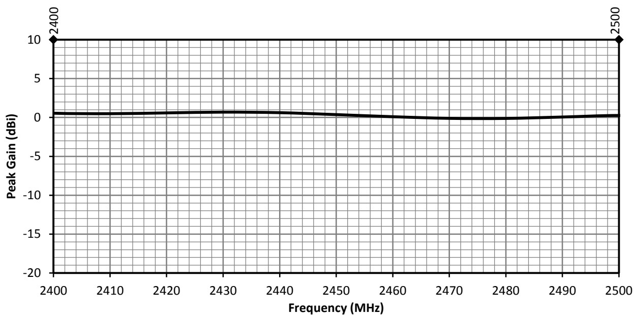
Figure 13. ANT-2.4-MMG1-SMA Antenna Peak Gain, Free Space
