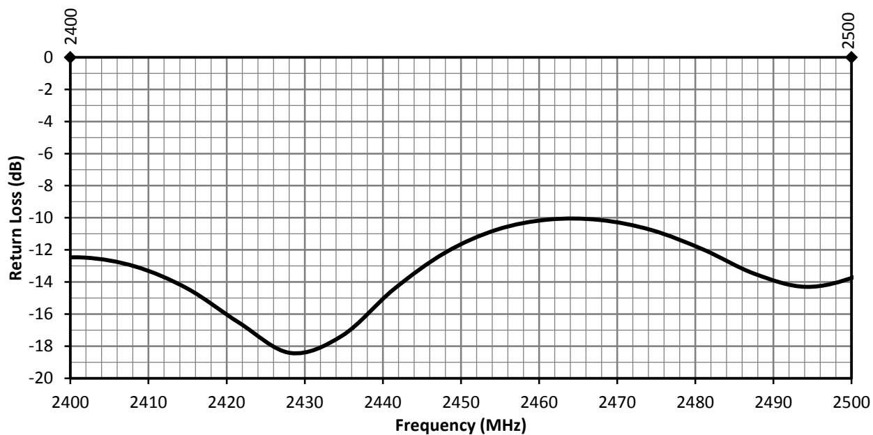
Figure 5. ANT-2.4-MMG1-SMA Antenna Return Loss on Ground Plane
