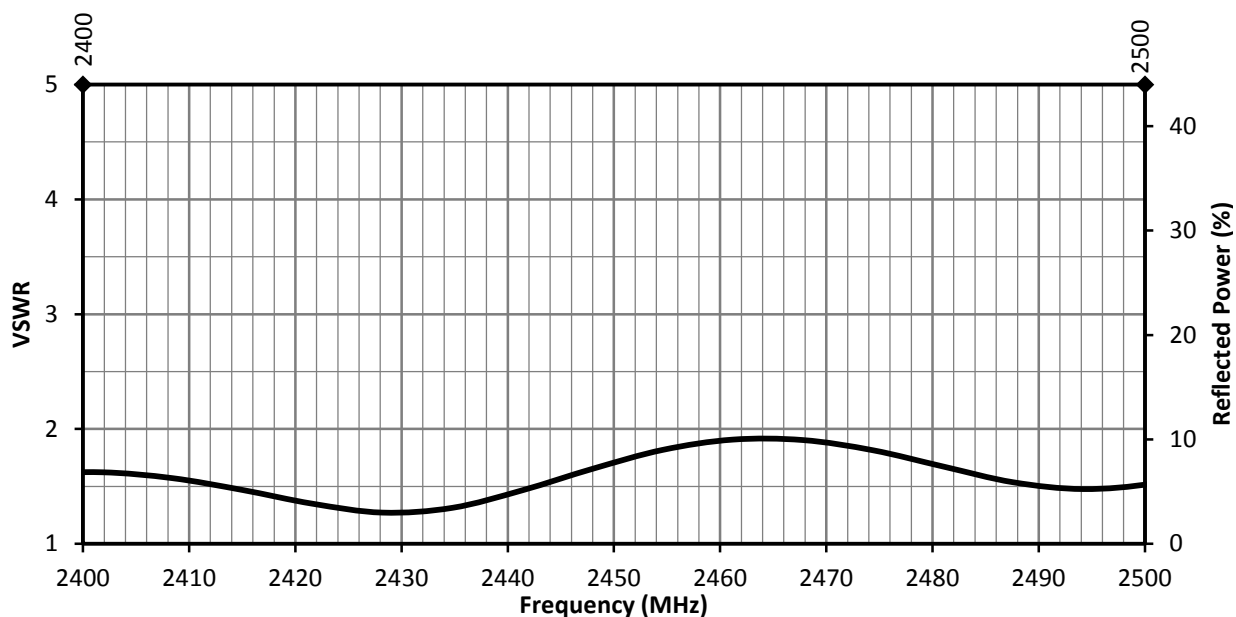
Figure 4. ANT-2.4-MMG1-SMA Antenna VSWR on Ground Plane
