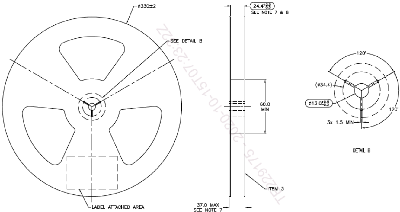
Tape & Reel – 150 pieces per reel
