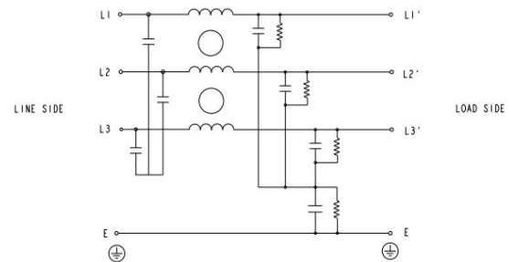
TYPICAL CIRCUIT DIAGRAM
