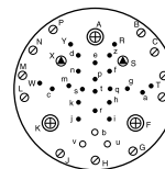
25-41 22 Size 22D Contacts 3 Size 20 Contacts 11 Size 16 Contacts 2 Size 12 Contacts 3 Size 8 Twinax
