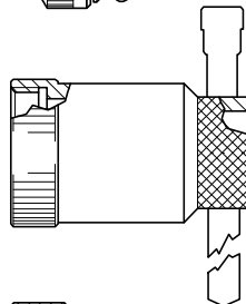
Backshell for Tinel-Lock Ring (Single Braid Cable)
