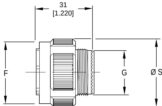
Plug Type 26
