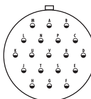
24-19 19#12 (I)
