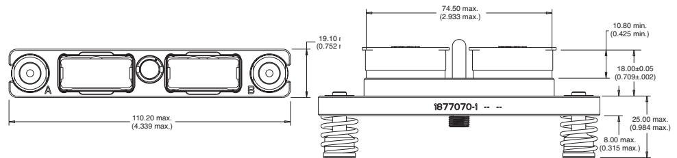
Plug Shell, Spring-Loaded, Float-Mounting GPR2 1877070-1
