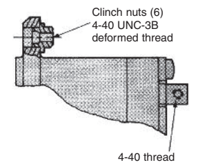
Modification 19 (RME, MME—threaded holes)
