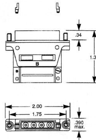
Socket-Cavity Receptacle Shell MTCR-103-04S
