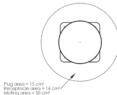
MIL-C-38999 21-35 fitted with 79x size 22 contacts
