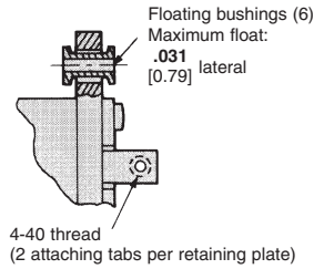
Modification 30 (R, RM, M, MM—attaching tabs)
