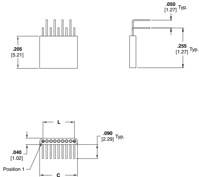
Plug Assembly Drawing Number 1589453
