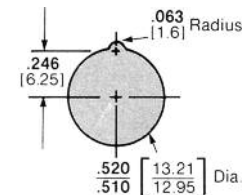
Recommended Panel Cutout for Bulkhead Mounting
