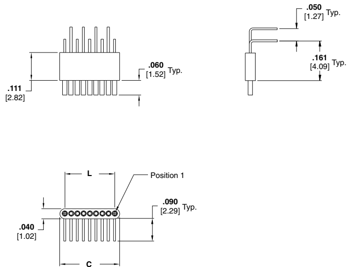
Receptacle Assembly Drawing Number 1589454
