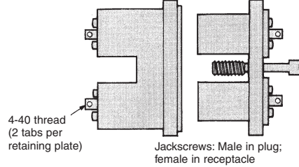
Modification 52 (R, RM, M, MM—attaching tabs)
