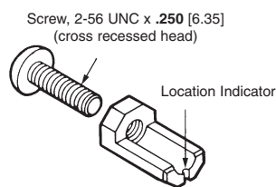
Kit Number 530341-7 (includes 2 keys and 2 screws)
