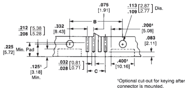
Straddle Mount Assembly
