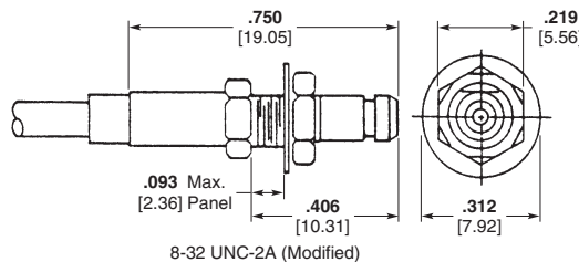
Bulkhead Jack, Rear Mount Part Number 145-0001-0001
