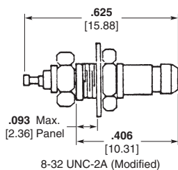
Receptacle, Rear Mount Part Number 145-0003-0001
