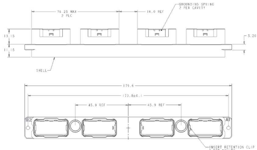
Receptacle, w/(2) thru holes 1996487-1
