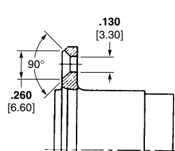
Modification 73 (without tabs) Modification 74 (with tabs) Size 1, 2, 3 shells — 4 c'sunk holes Size 4 shells — 6 c'sunk holes
