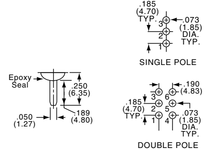
Printed Circuit
