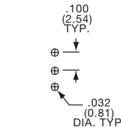
P.C. HOLE LAYOUT SINGLE POLE
