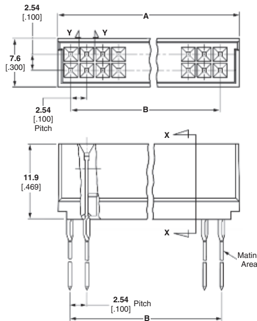
Section Y-Y
