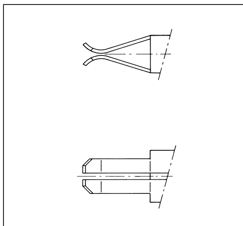
Junior Timer Contact – Modified – Chamfered Springs
