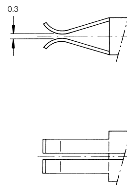
Junior Timer Contact – Special Version – Gap Size = 0.3 mm
