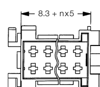
Tab Housing
