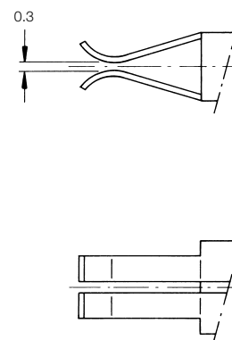
Junior Timer Contact – Special Version –
