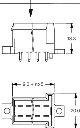
Pin Header 180°
