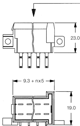
Pin Header 90°
