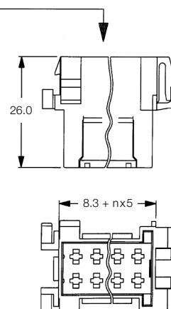
Tab Housing
