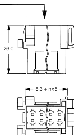
Tab Housing
