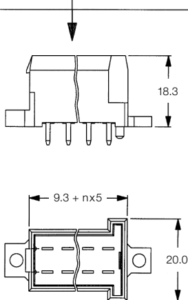
Pin Header 180°
