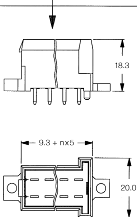
Pin Header 180°
