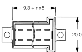
Pin Header 180°
