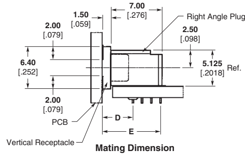
Mating Dimension
