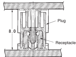
Part No.: 5177983-□ (Page 78) 8 [.315] Stacking Height
