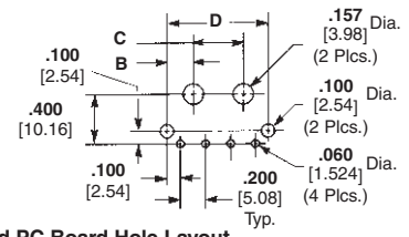
Recommended PC Board Hole Layout .062 [1.57] thick PC Board
