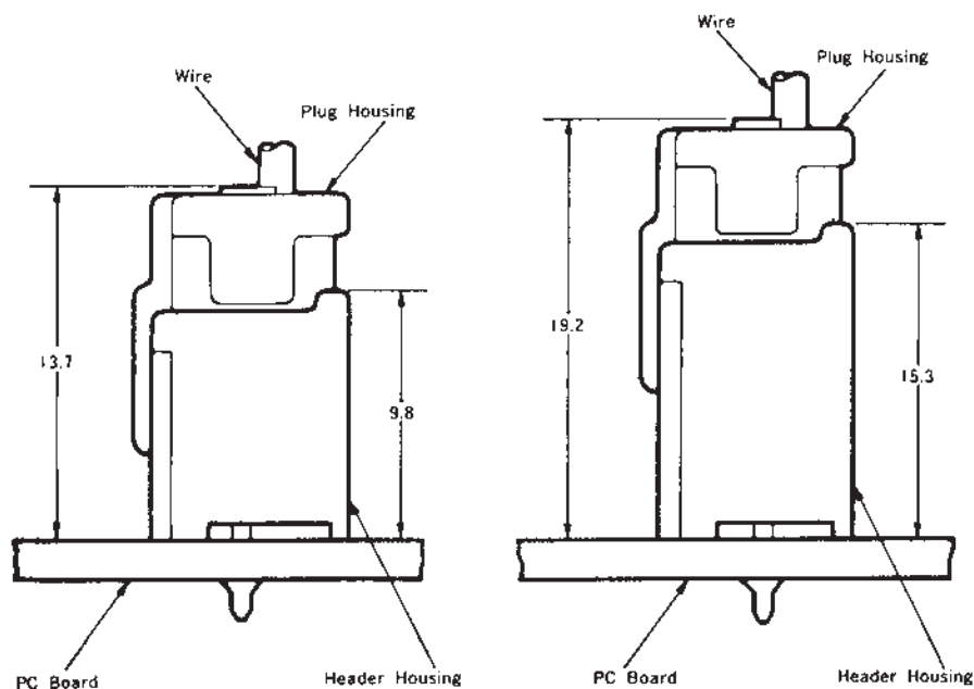
Standard-Profile Type
