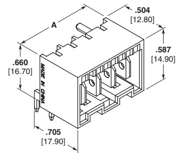
Right-Angle Orientation
