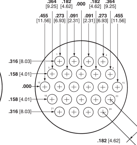
Arrangement 23-24 Max. Wire Ins. Dia. = .150 [3.81]
