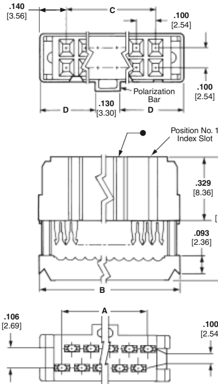
Housing Assembly and Cover
