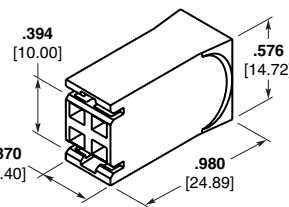
Two Circuit Wax Motor Housing
