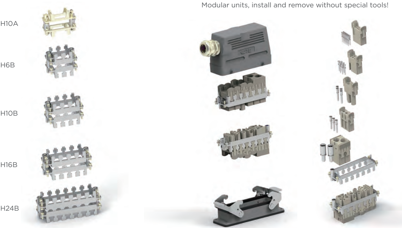
HMN module fixing frame
