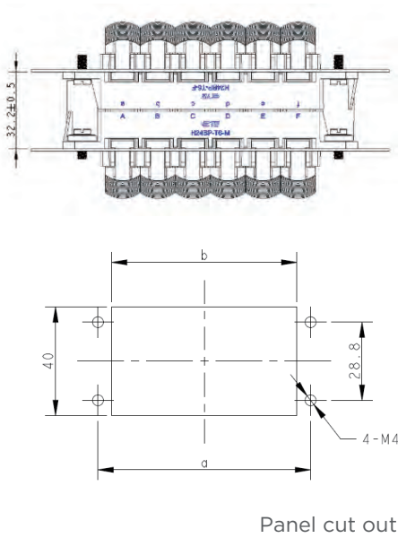
Space of two Panels at close status
