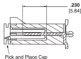
Section K-K
