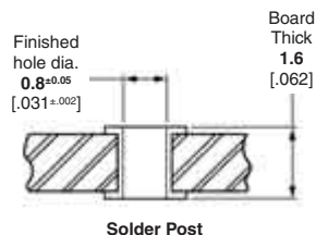
Solder Post
