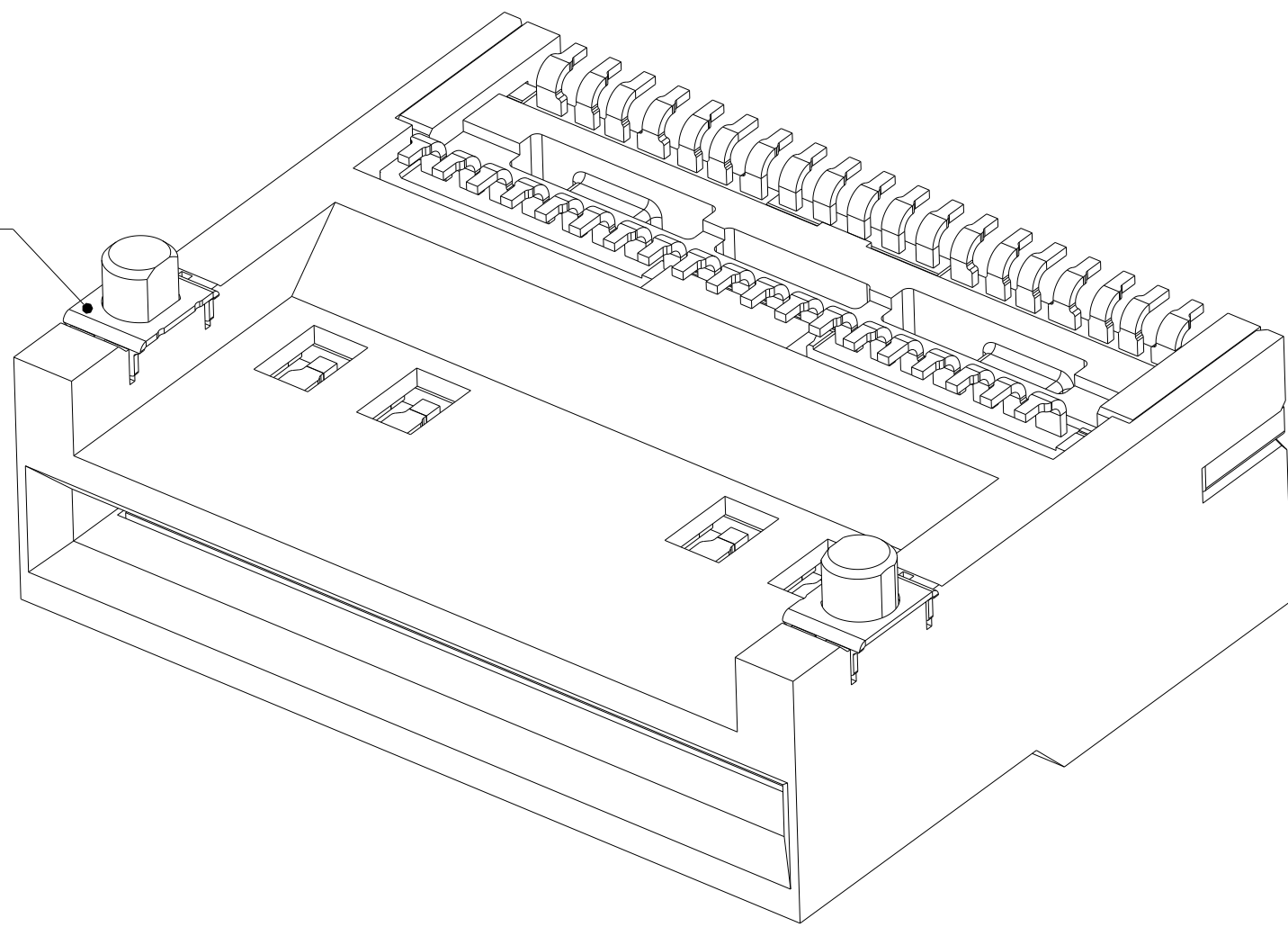
2401838-2 AND -4 SCALE 8:1
