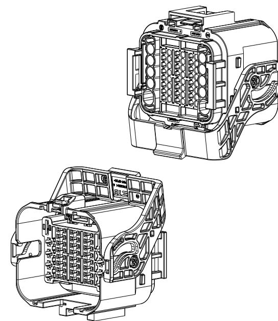
DELIVERY CONDITION OF SEC LOCK IN PRE LOCKED CONDITION
