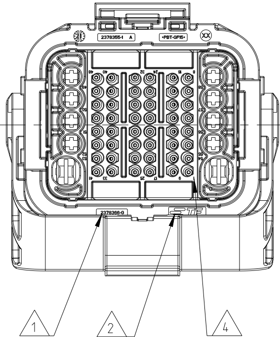
DELIVERY CONDITION OF SEC LOCK IN PRE LOCKED CONDITION
