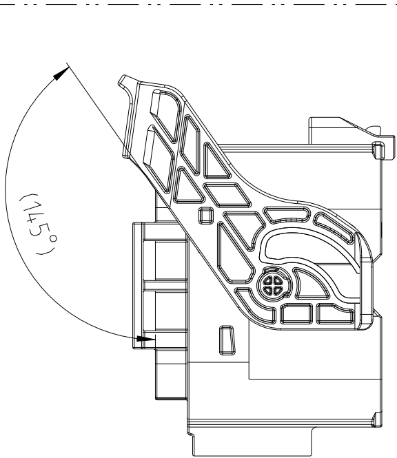
8 LEVER PRE-LOCK CONDITION
