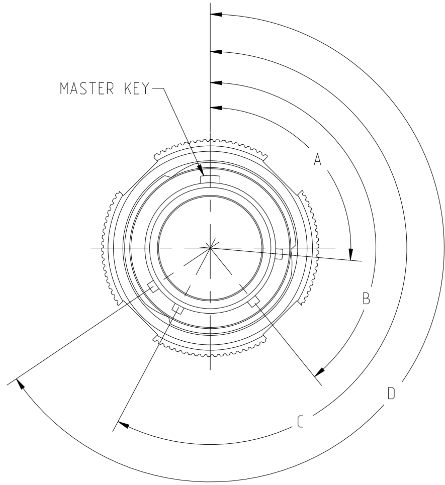
KEYING ORIENTATION DETAIL
