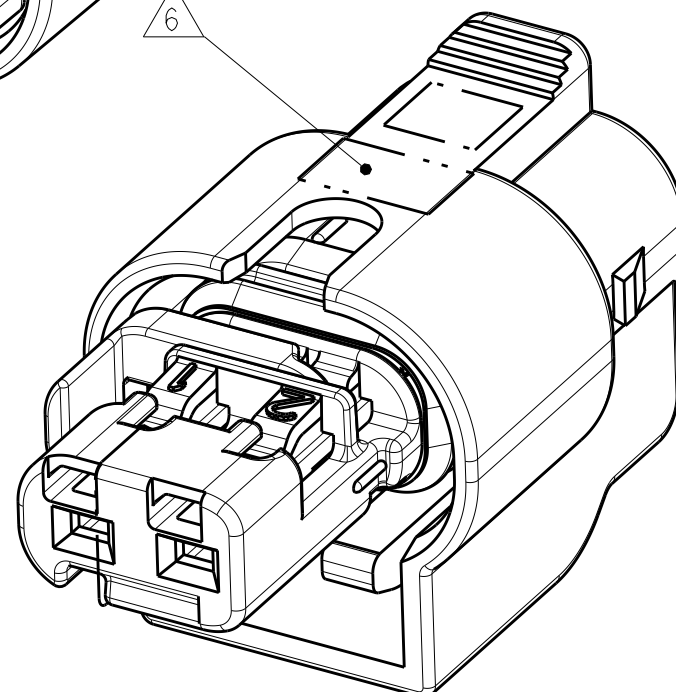
ISOMETRIC VIEWS 2098557-4
