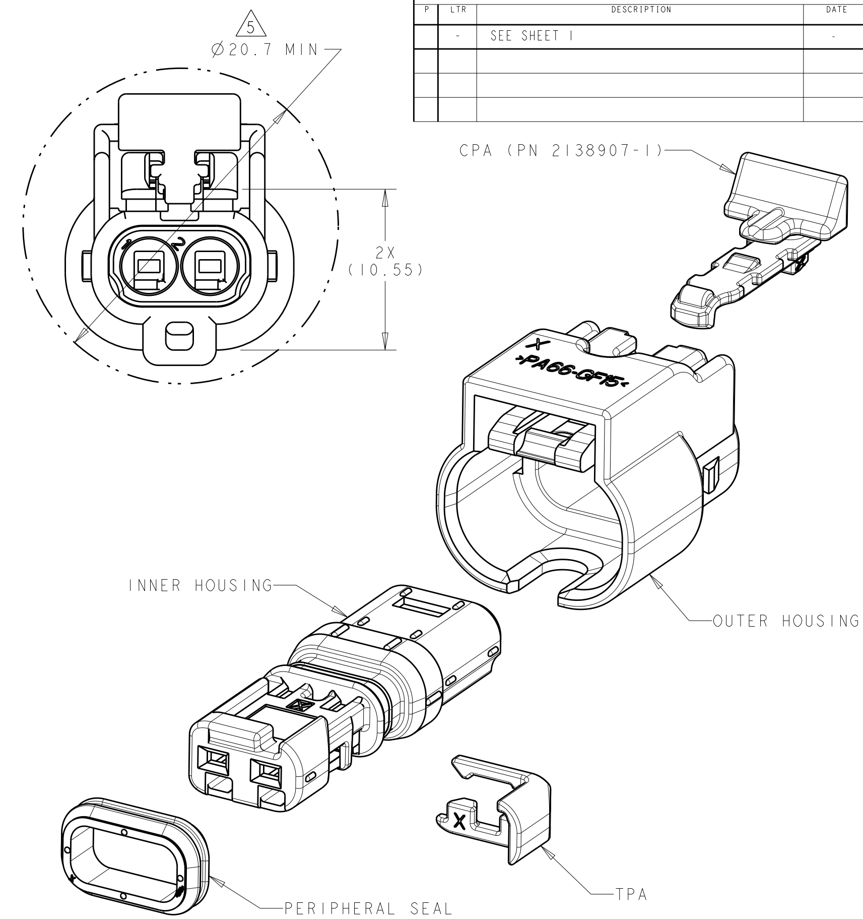
4-2098557-1 EXPLODED ISOMETRIC VIEW
