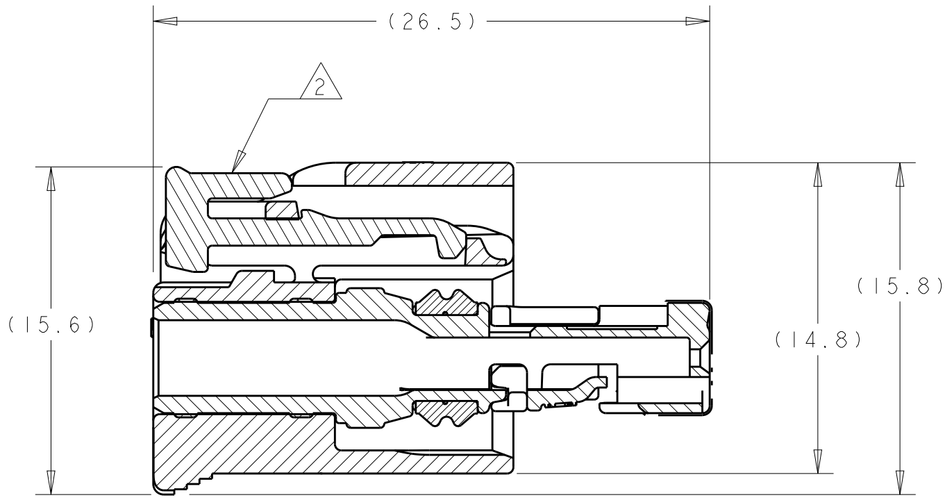
SECTION B-B
