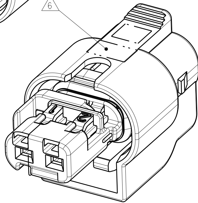
ISOMETRIC VIEWS 2098557-4
