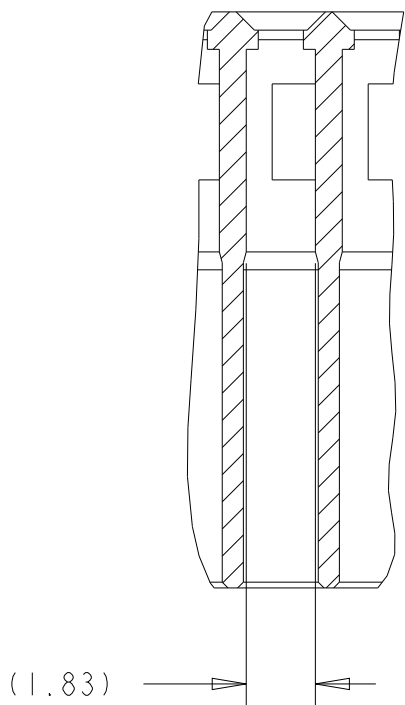
SECTION Y-Y
